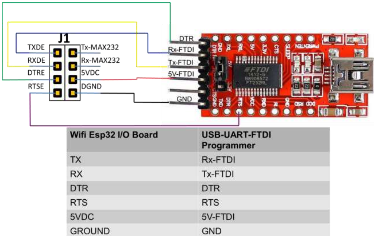
Figure 7: Programmer Connection Diagram
