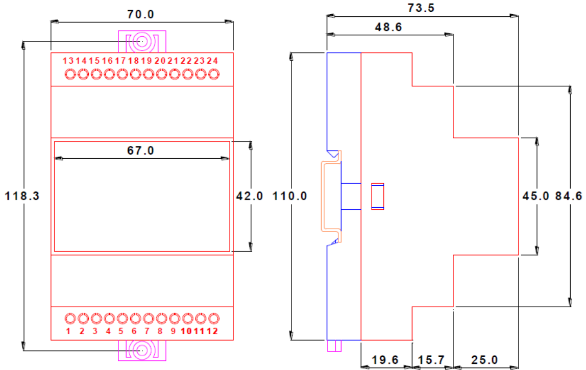
Figure 2: Board Dimensions
